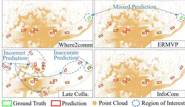
Figure 3: Qualitative comparison on OPV2V dataset.
